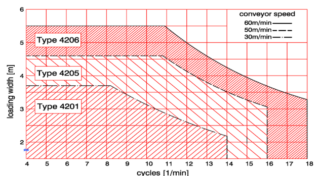
Range of application of diverse Heye Lehr Loaders
