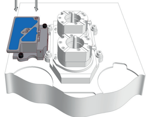
Conversion from axial to radial cooling (6 1/4" DG)
